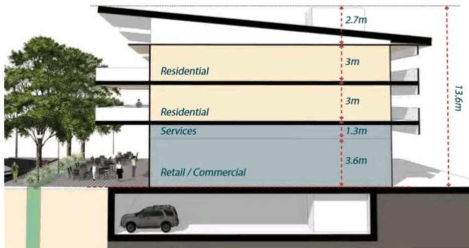
Figure 1: Example of a three storey commercial / residential building and height
